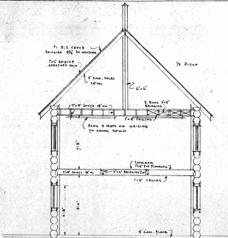
SECTION SCALE 1/4" = 1'-0"
