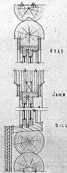
DETAIL OF 2 ND FLOOR WINDOWS SCALE 1/2" = 1'-0"
