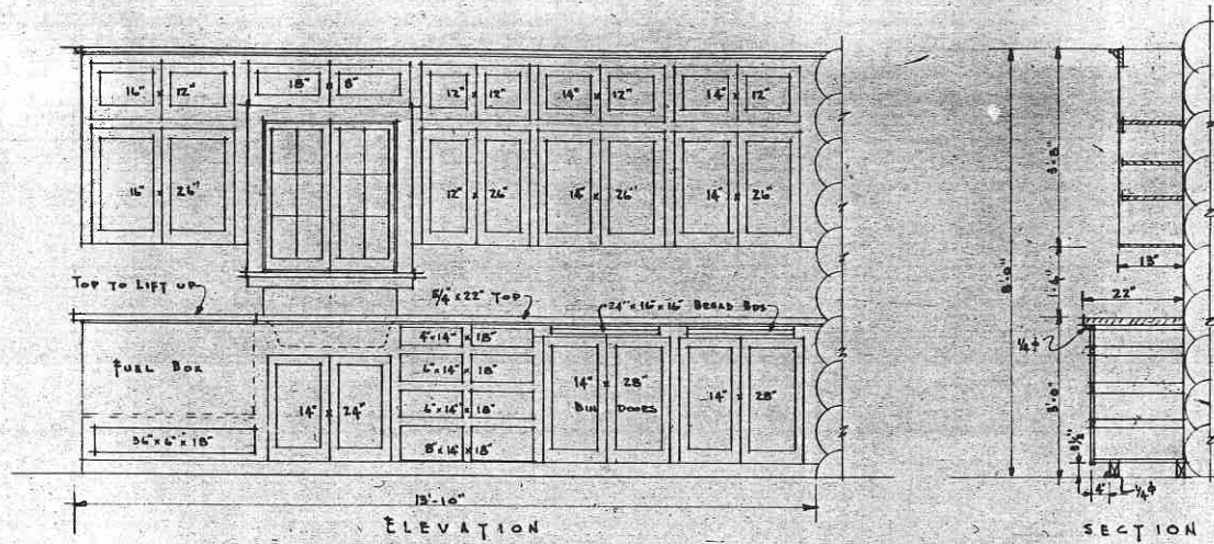
KITCHEN CABINET DETAILS SCALE 1/2" = 1'-0"
