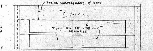
DETAIL OF BED SCALE 3/4" = 1'-0"
