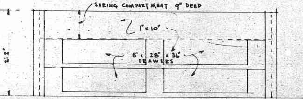
DETAIL OF BED SCALE 3/4" = 1'-0"
