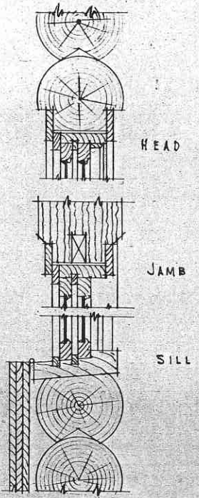
DETAIL OF 2 ND FLOOR WINDOWS SCALE 1/2" = 1'-0"
