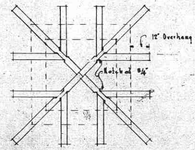
TOP VIEW SHOWING ROOF FRAMING All roof members to 4" diam. poles
