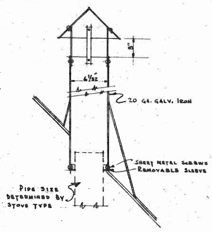
SECTION THRU SAFETY THIMBLE & FLUE SCALE 1/2" = 1'-0"
