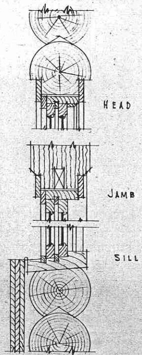
DETAIL OF 2 nd FLOOR WINDOWS SCALE 1 1/2" = 1'-0"
