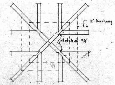
TOP VIEW SHOWING ROOF FRAMING All roof members to 4" diam. poles
