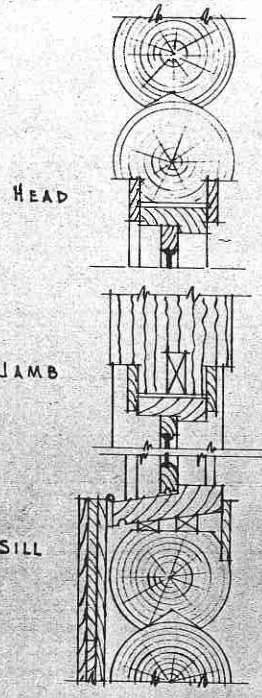
DETAIL OF 1 st FLOOR WINDOWS SCALE 1 1/2" = 1'-0"
