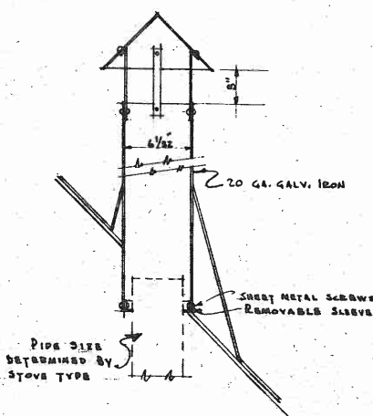
SECTION THRU SAFETY THIMBLE & FLUE SCALE 1/2" = 1'-0"
