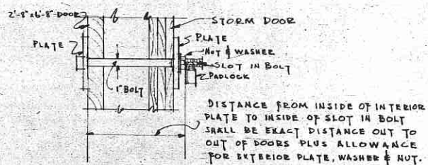
DOOR LOCKING BOLT SCALE 1 1/2" = 1'-0"
