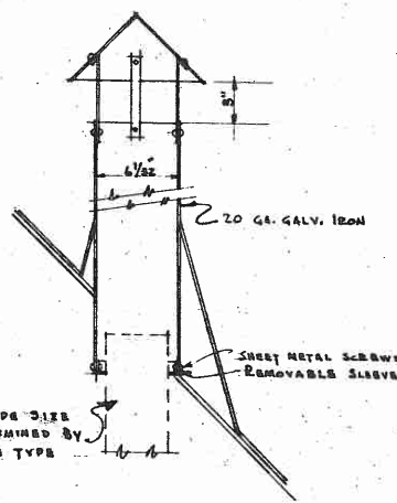
SECTION THRU SAFETY THIMBLE & FLUE SCALE 1/2" = 1'-0"
