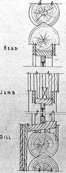
DETAIL OF 1 ST FLOOR WINDOWS SCALE 1/2" = 1'-0"
