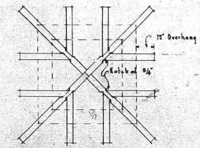
TOP VIEW SHOWING ROOF FRAMING All roof members to 4\"/>
