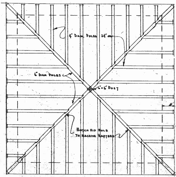
REFLECTED VIEW OF ROOF CONSTRUCTION SCALE 1/4" = 1'-0"
