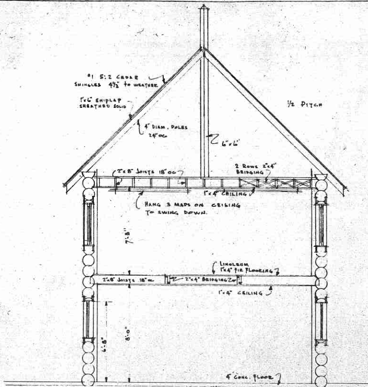
SECTION SCALE 1/4" = 1'-0"
