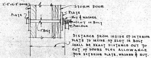
DOOR LOCKING BOLT SCALE 1 1/4" = 1'-0"
